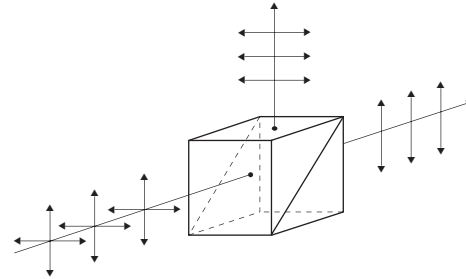
Figure 4 Example of a Polarizing Beamsplitter Cube.
